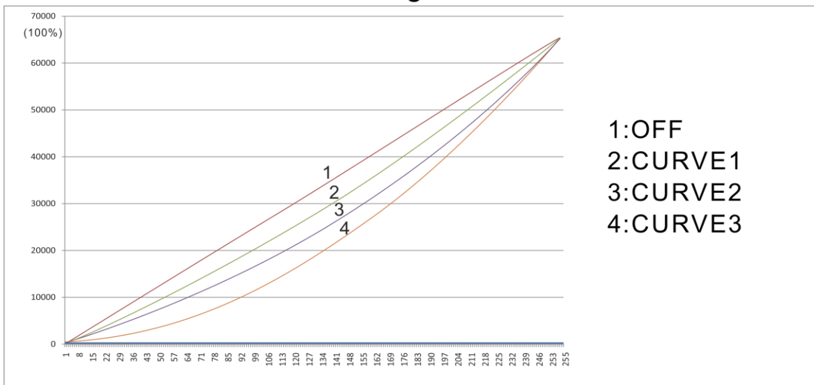
Dimming curves
