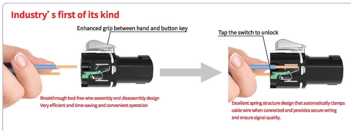
Figure Showing Tool-free Wiring Design
