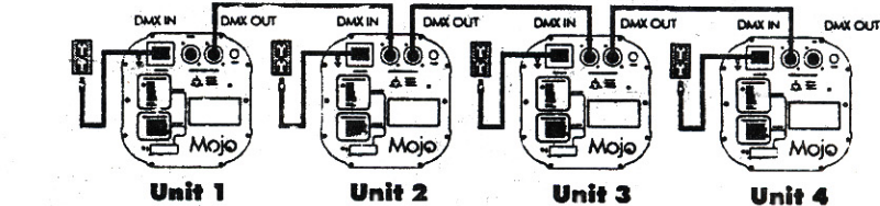
DMX Set Up - MJS-1
